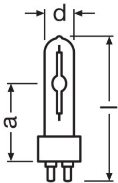
HCL-T 35 W/942 NDL PB
